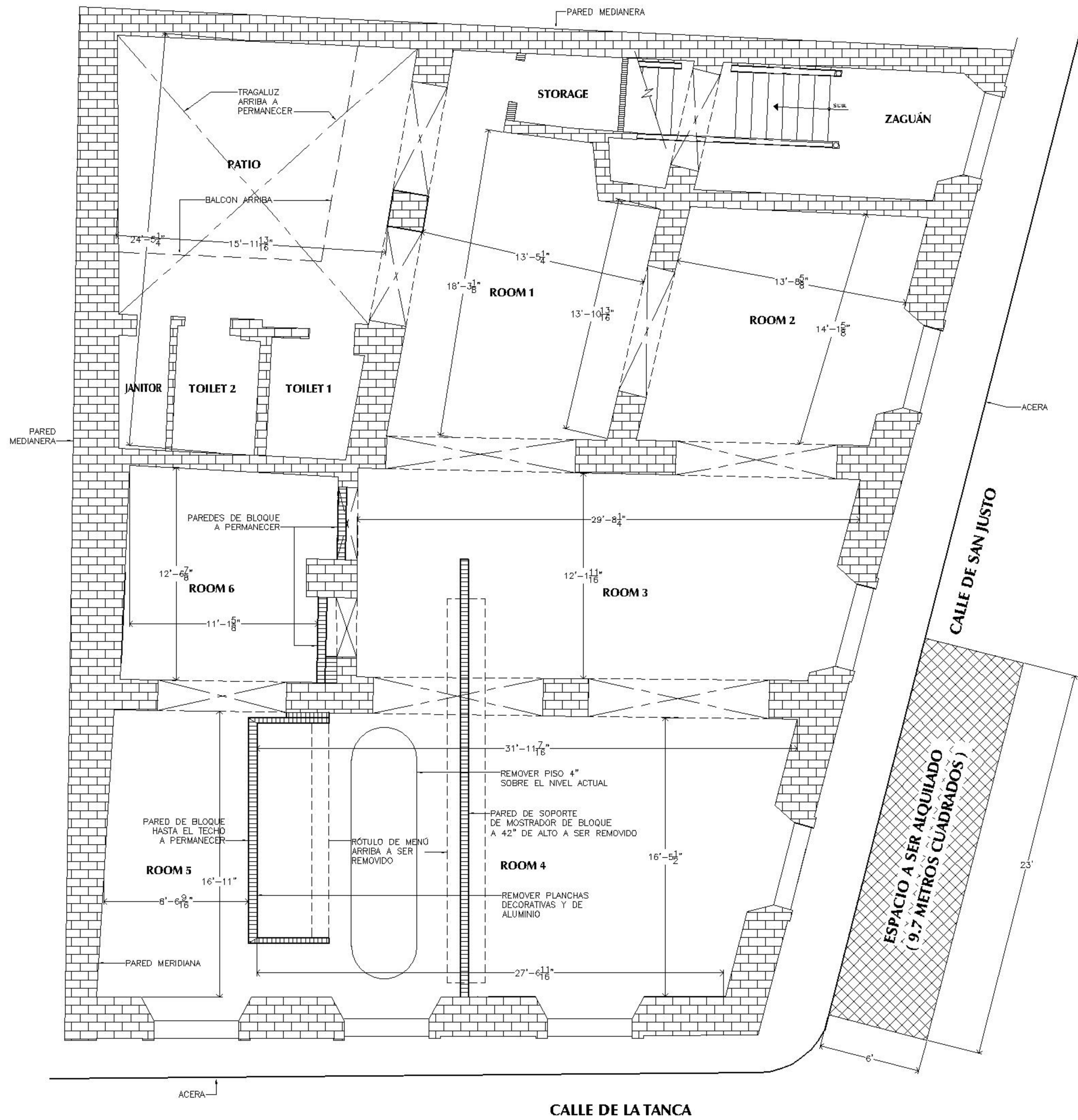
ORIGINAL STATE OF BUILDING GROUND FLOOR LEVEL BEFORE REHABILITATED FOR A FAST FOOD RESTAURANT
